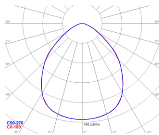
FUTURA NT-60x60_-45W_mP
